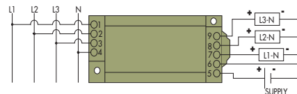
CR4880 3 Element, 4 Wire - 4 - 20 mA DC Output
