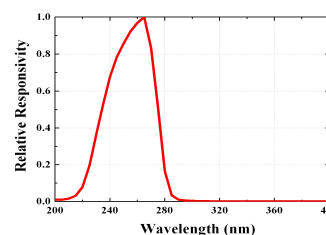
Fig. 2 Responsivity Curve
