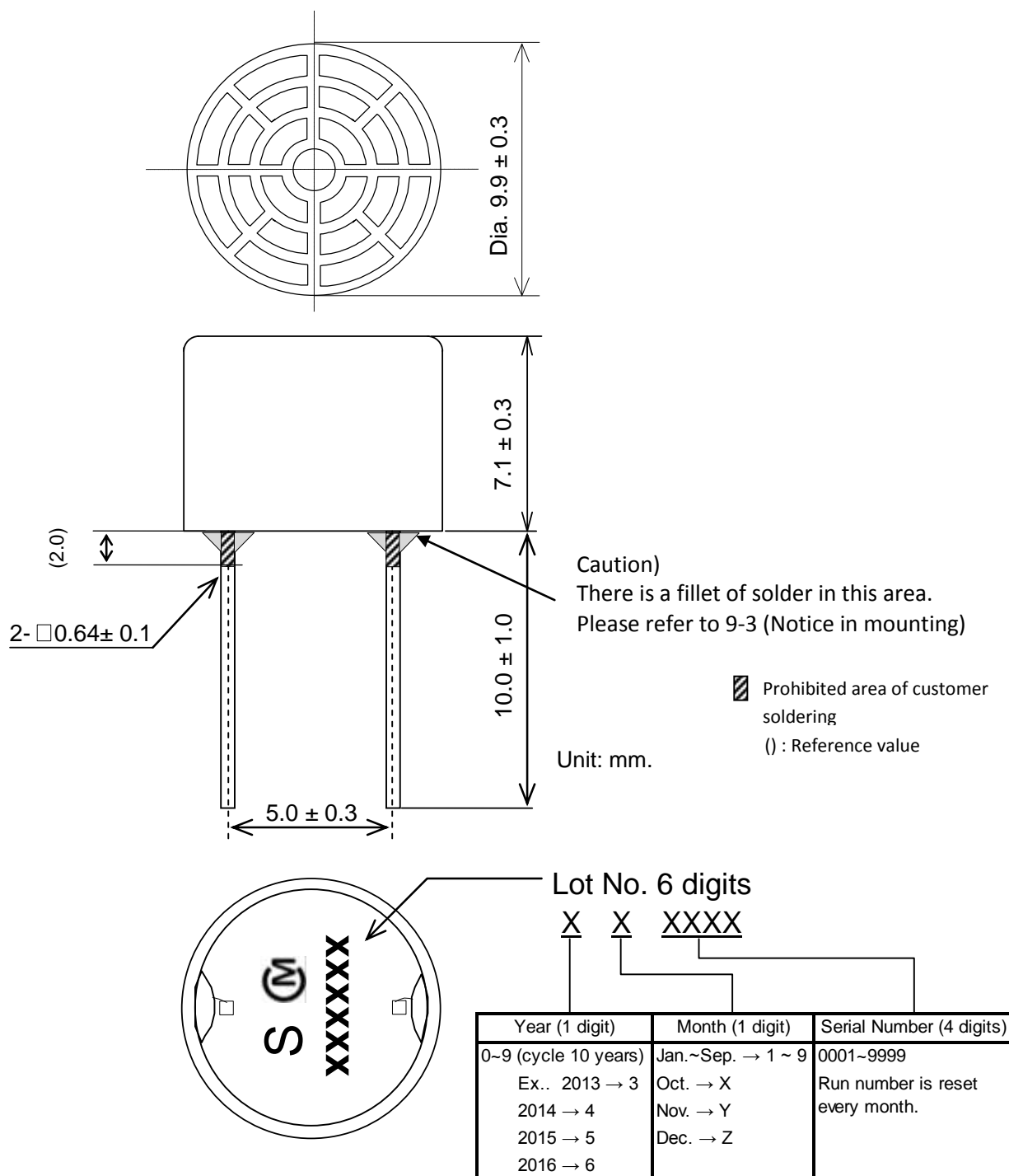
Fig.1: Product Dimension
