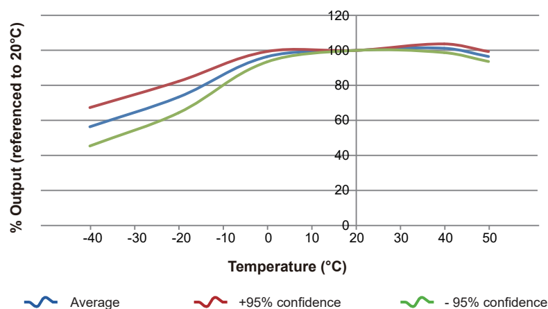
Temperature Performance of WC Air Quality Sensor
